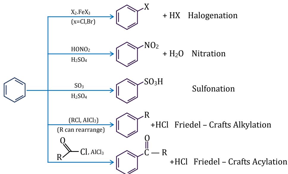
Electrophilic Aromatic Substitution Reactions
